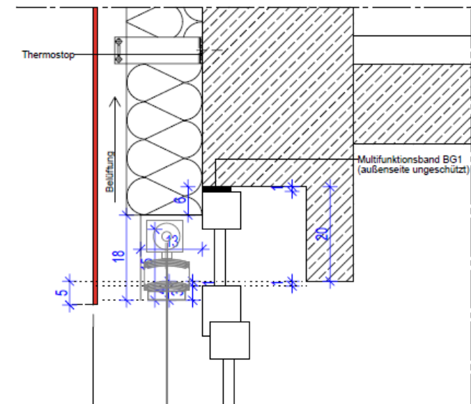
Detail 1
